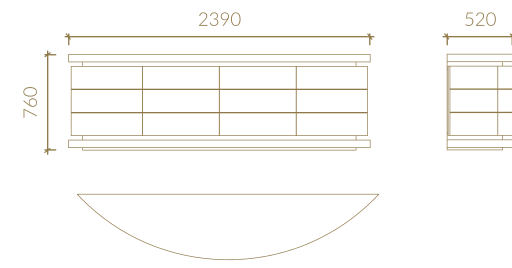
4 DOORS SIDEBOARD
