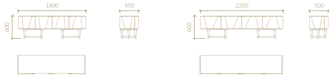
TV UNIT
