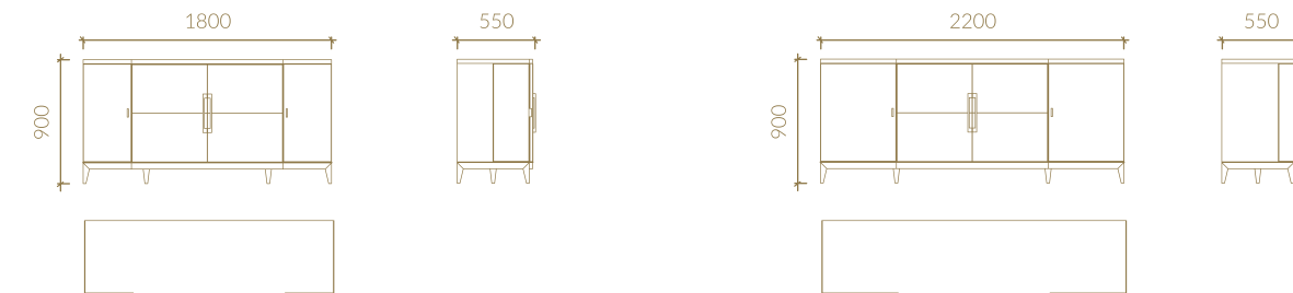
SIDEBOARD
