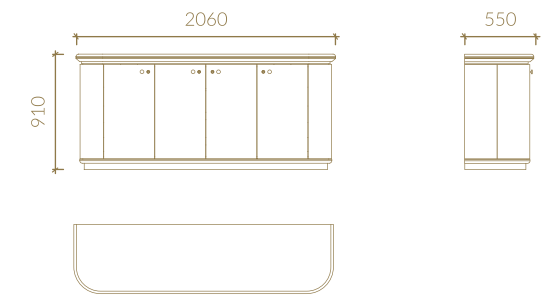
SIDEBOARD
