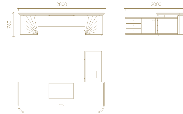
DESK
