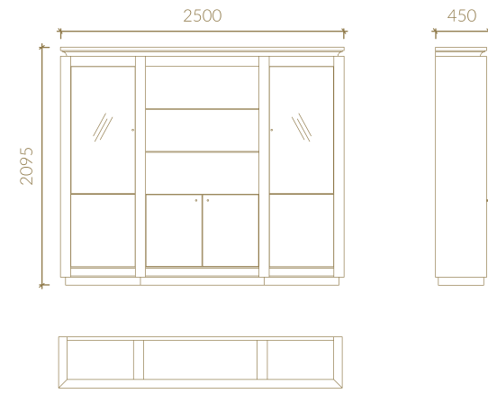
LIBRARY
