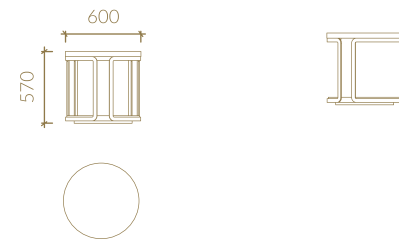
SUPPORT TABLE
