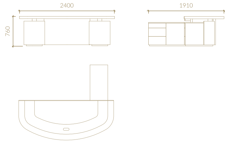
DESK
