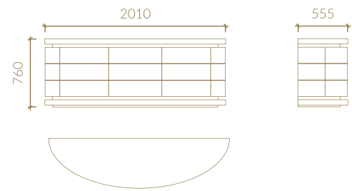
3 DOORS SIDEBOARD
