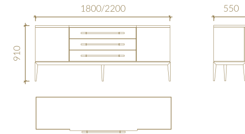
SIDEBOARD
